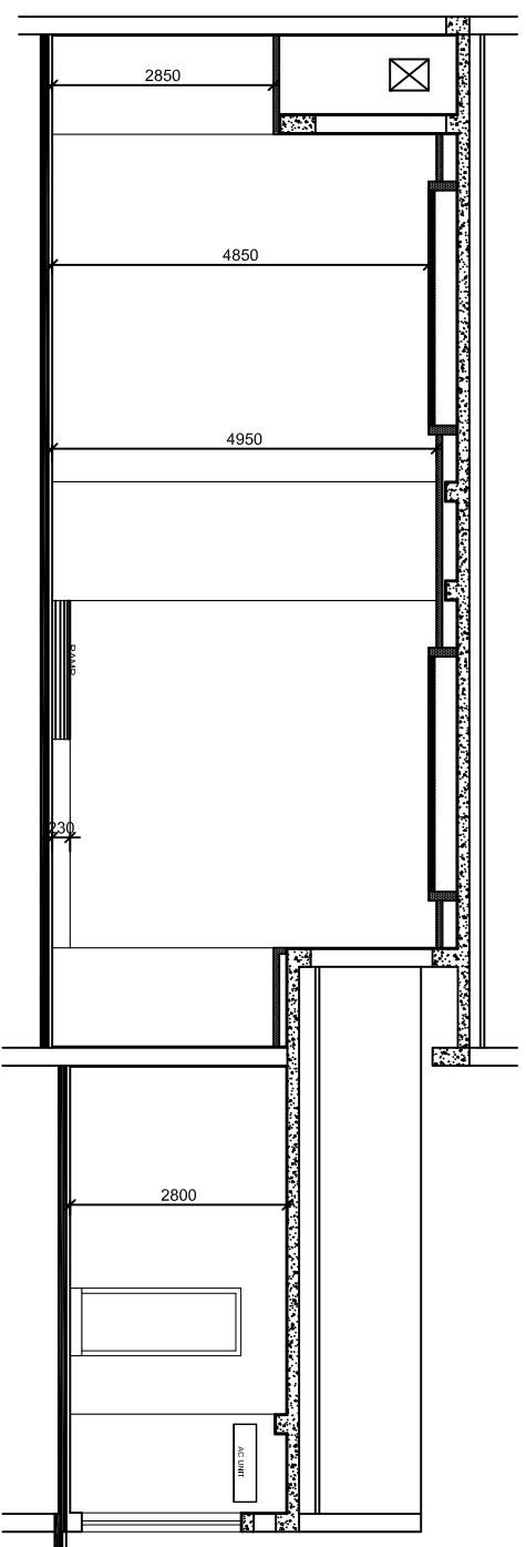
SECTION 1-1
